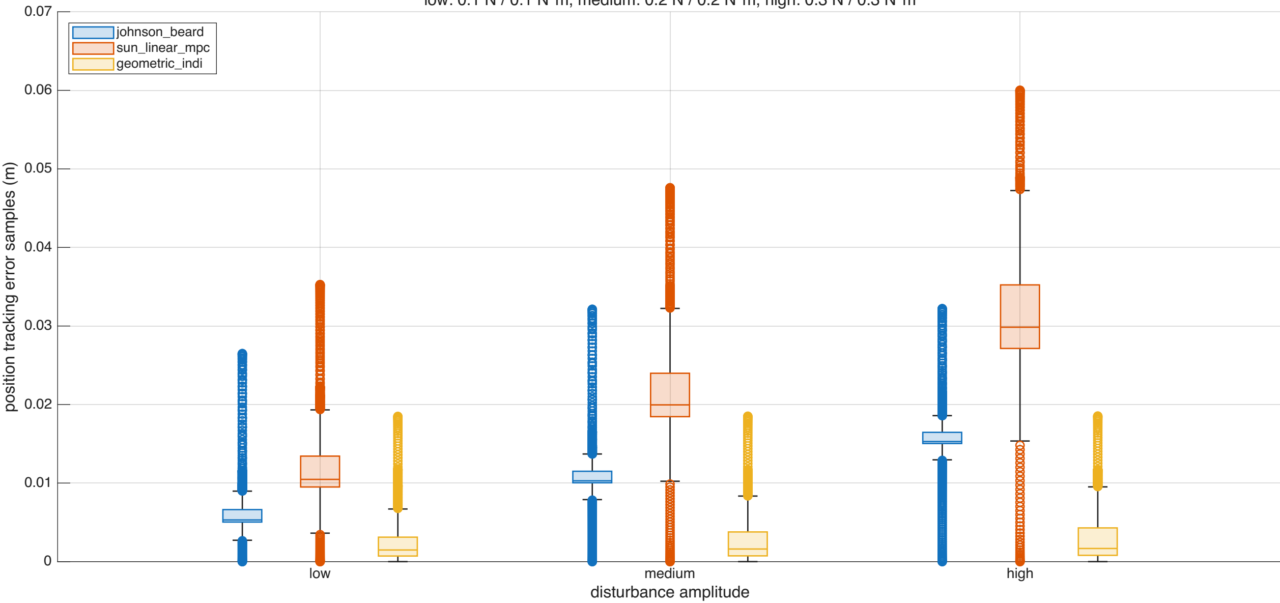
Trajectory: helix_flip low: 0.1 N / 0.1 N*m, medium: 0.2 N / 0.2 N*m, high: 0.3 N / 0.3 N*m
